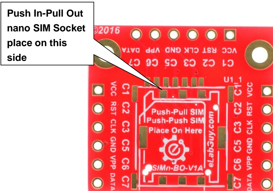
Figure 4: SIMn-PSPL-BO-V1A PCB
