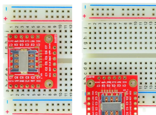
Figure 2: Example of connecting the SIMn-PSPL-BO-V1A on a breadboard
